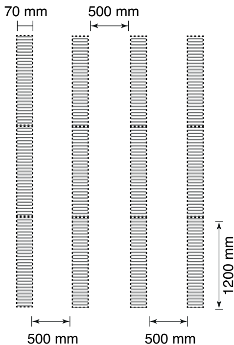
Equivalent sound absorption area per element A obj
